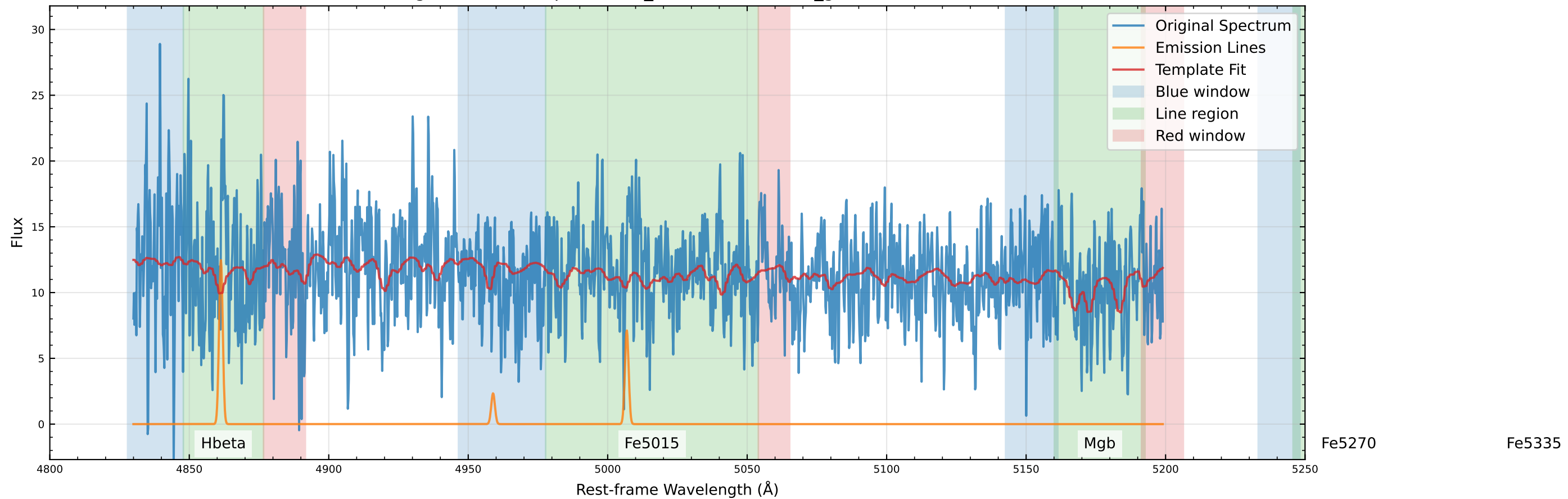
Original Data Comparison (v_star=67.4 km/s, v_gas=59.3 km/s)
