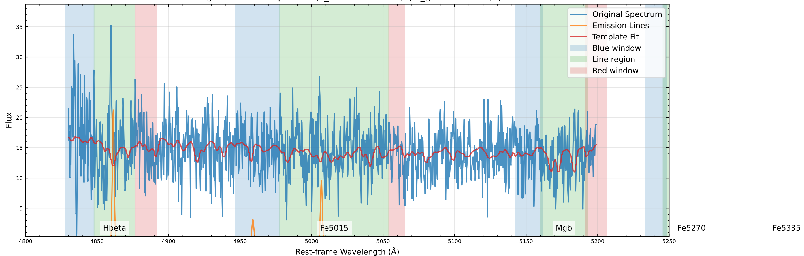
Original Data Comparison (v_star=-116.2 km/s, v_gas=-98.3 km/s)
