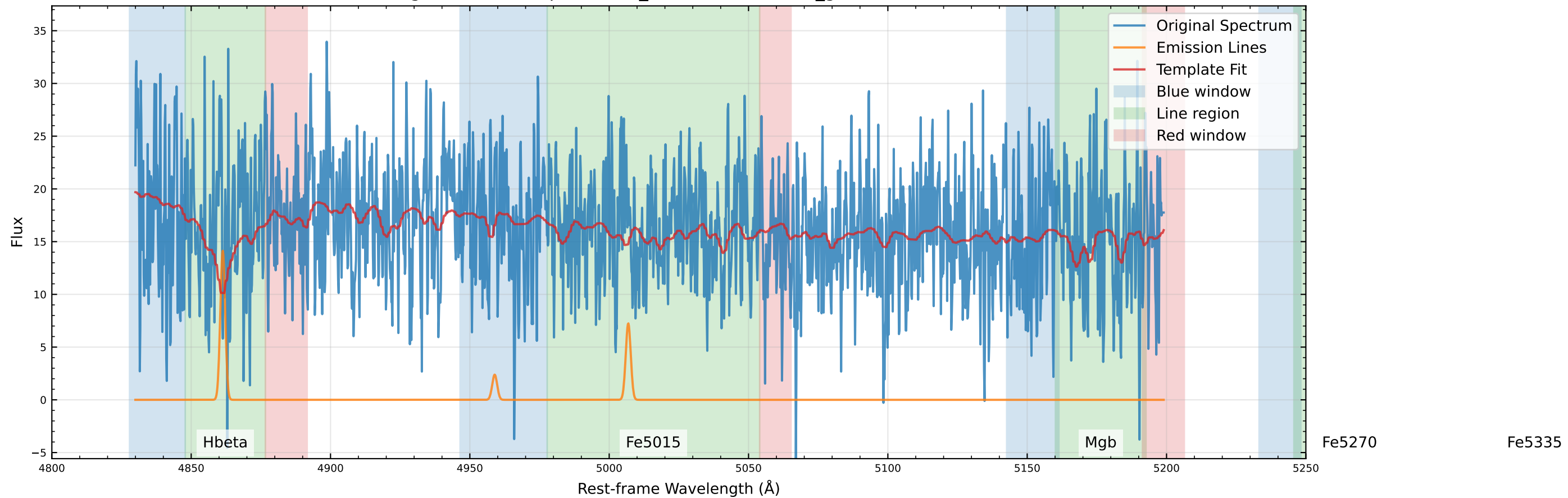
Original Data Comparison ( v_{\text{star}}=-62.7 km/s, v_{\text{gas}}=-78.4 km/s)
