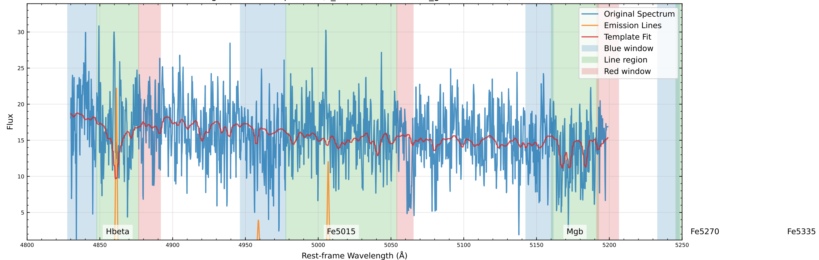
Original Data Comparison (v_star=-102.0 km/s, v_gas=-96.4 km/s)
