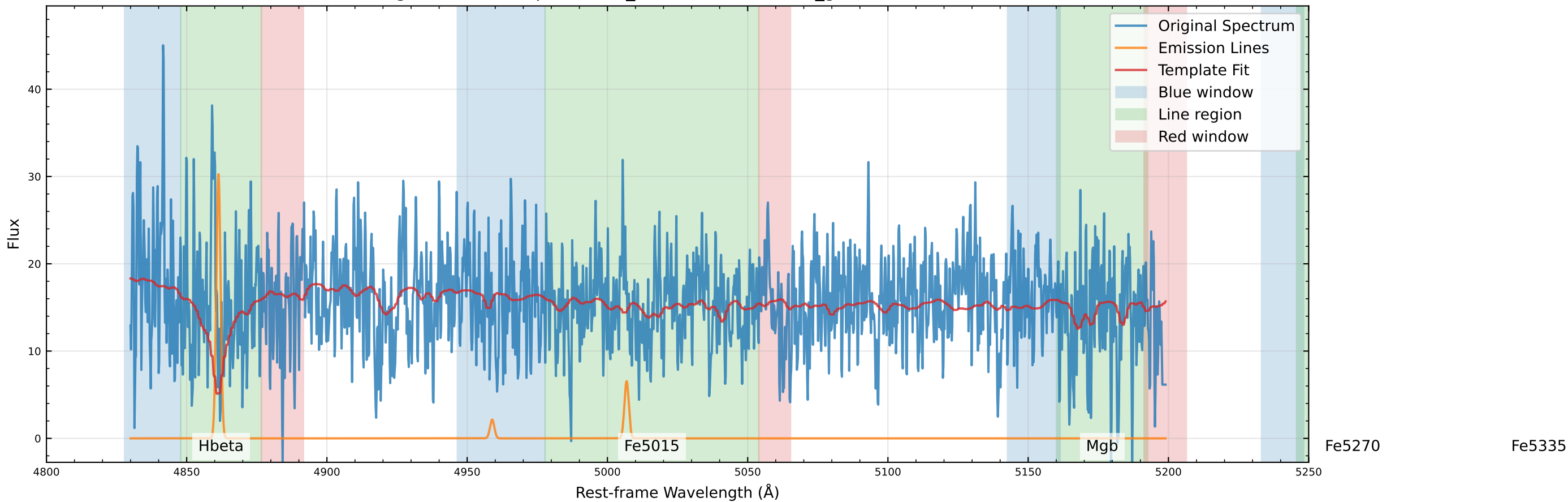
Original Data Comparison (v_star=-150.2 km/s, v_gas=-114.3 km/s)
