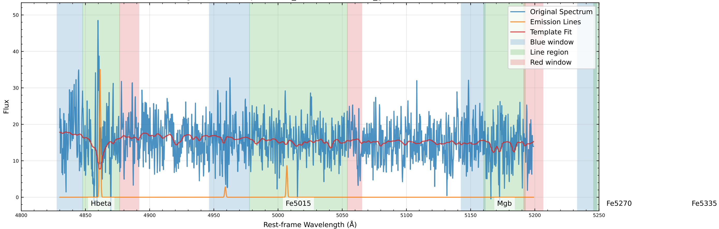
Original Data Comparison (v_star=-58.2 km/s, v_gas=-77.0 km/s)
