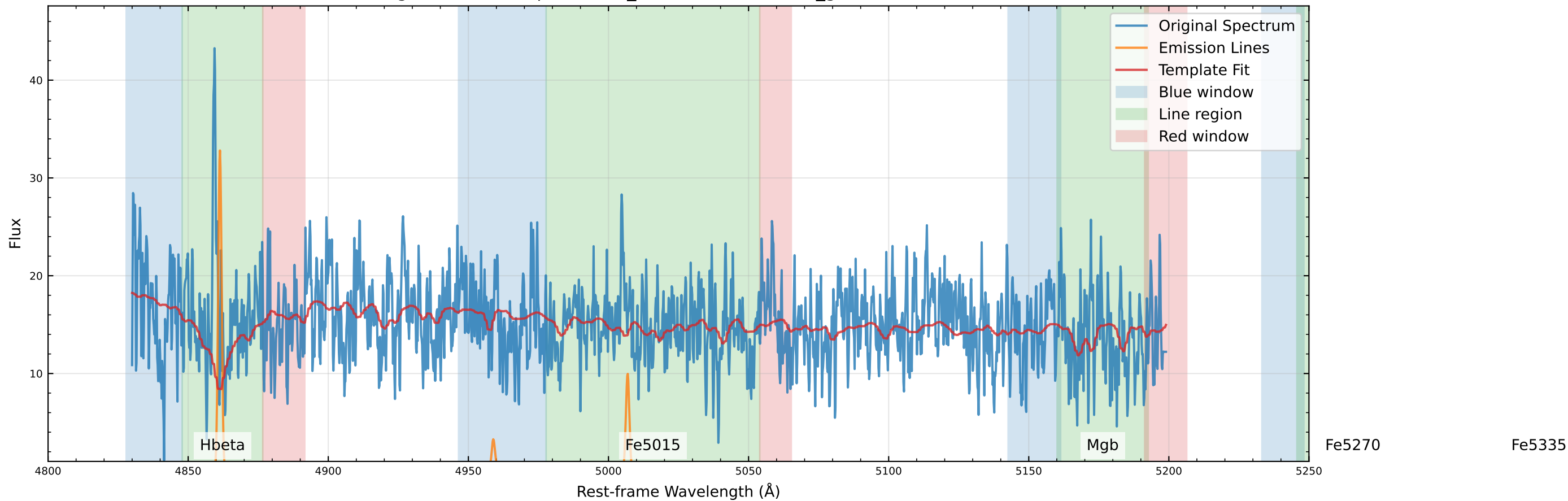
Original Data Comparison (v_star=-133.8 km/s, v_gas=-118.5 km/s)
