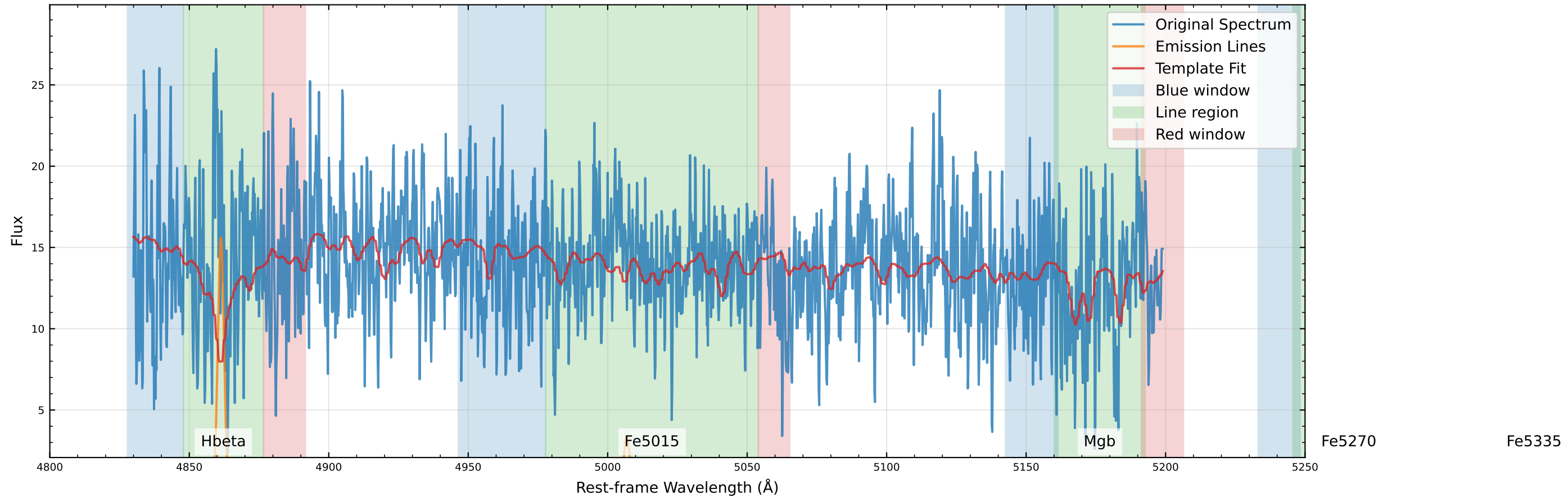
Original Data Comparison ( v_{\text{star}}=-95.2 km/s, v_{\text{gas}}=-97.1 km/s)
