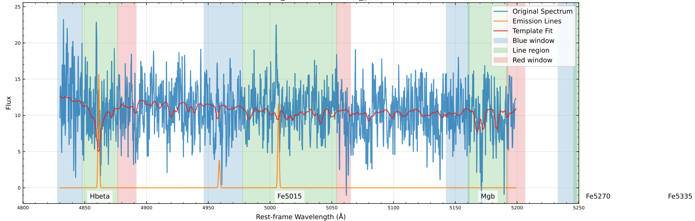
Original Data Comparison (v_star=-83.7 km/s, v_gas=-109.1 km/s)
