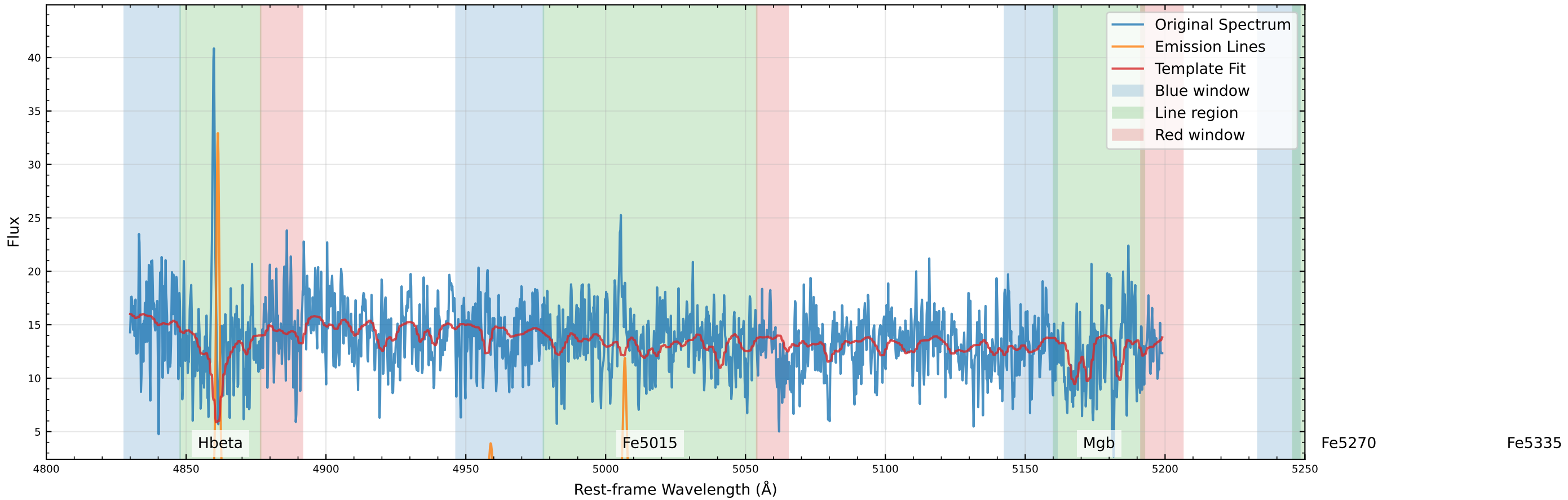
Original Data Comparison (v_star=-75.0 km/s, v_gas=-91.8 km/s)
