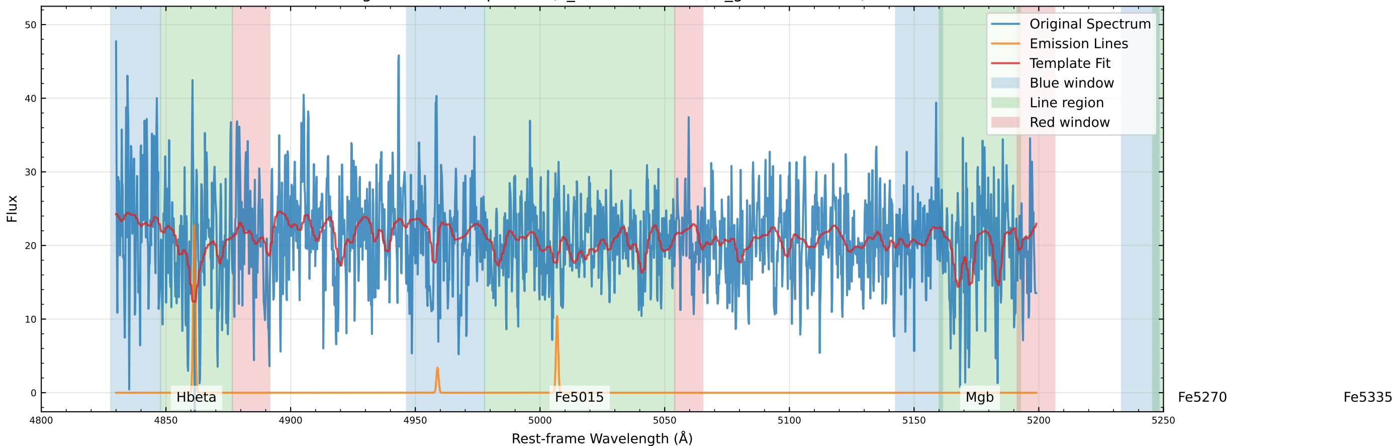
Original Data Comparison (v_star=-56.6 km/s, v_gas=-45.6 km/s)
