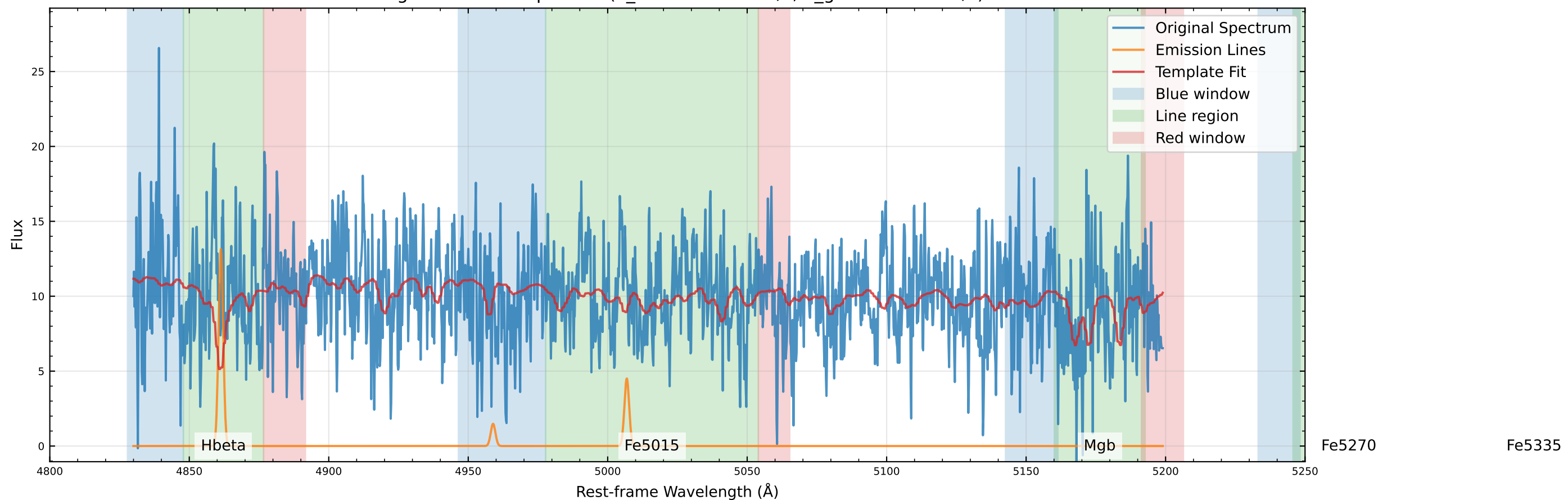
Original Data Comparison (v_star=-176.5 km/s, v_gas=-151.6 km/s)
