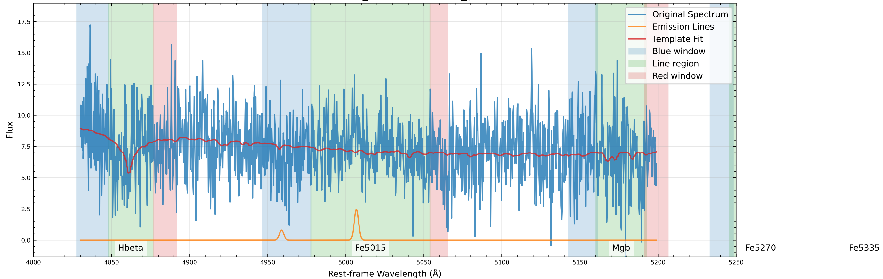
Original Data Comparison (v_star=-55.9 km/s, v_gas=-67.6 km/s)
