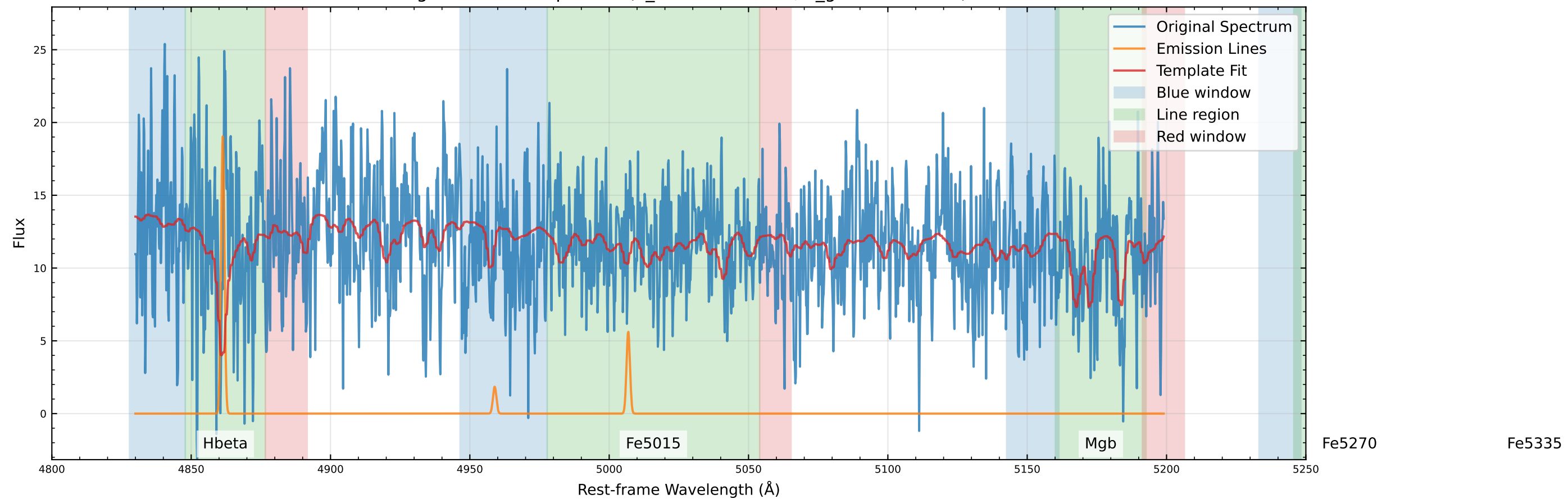
Original Data Comparison (v_star=49.5 km/s, v_gas=54.0 km/s)
