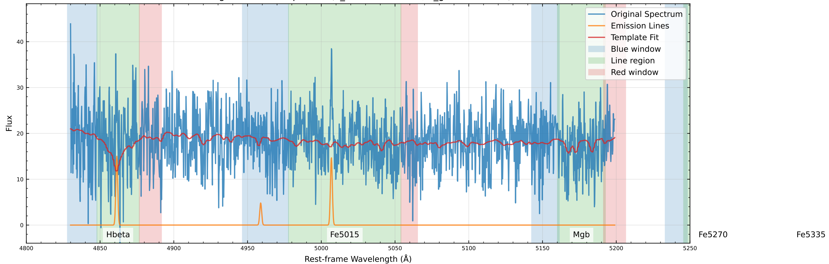
Original Data Comparison (v_star=-43.2 km/s, v_gas=-2.6 km/s)
