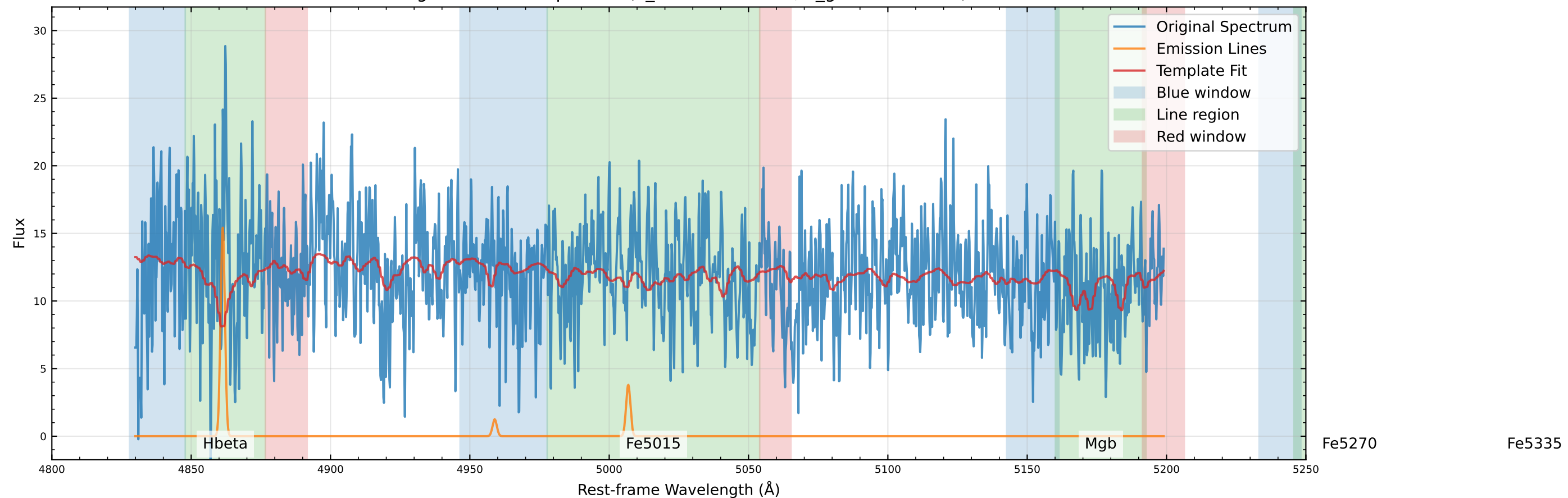
Original Data Comparison (v_star=62.3 km/s, v_gas=60.9 km/s)
