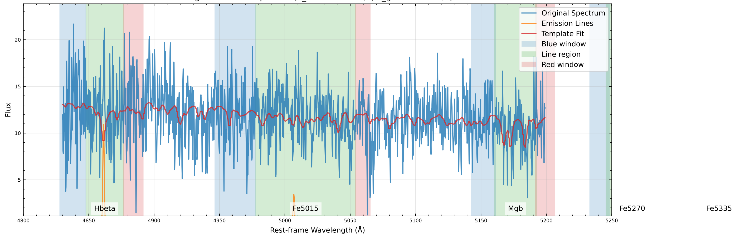
Original Data Comparison (v_star=67.3 km/s, v_gas=30.9 km/s)
