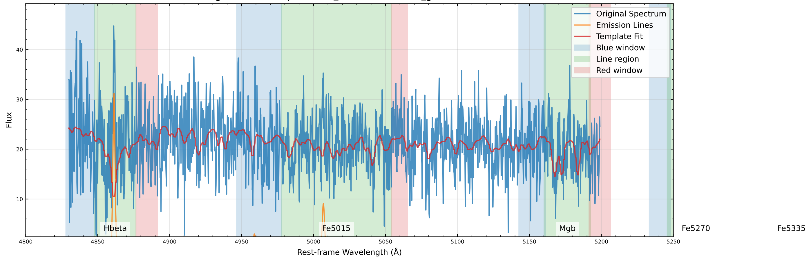
Original Data Comparison (v_star=23.1 km/s, v_gas=-0.7 km/s)
