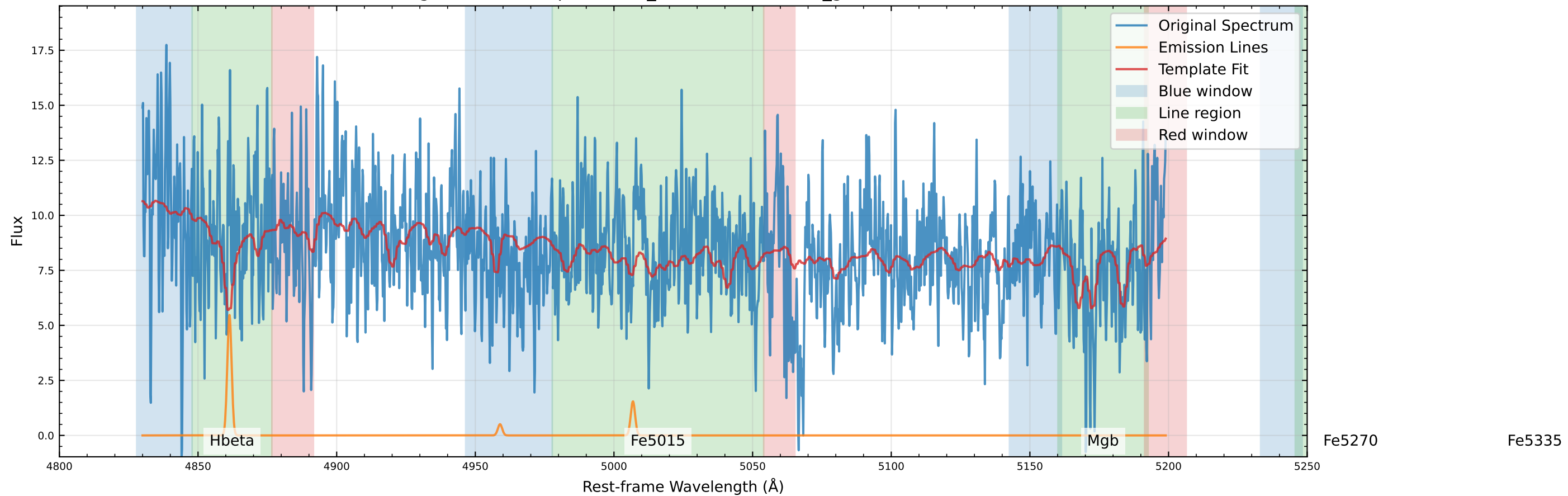
Original Data Comparison (v_star=-22.7 km/s, v_gas=13.1 km/s)
