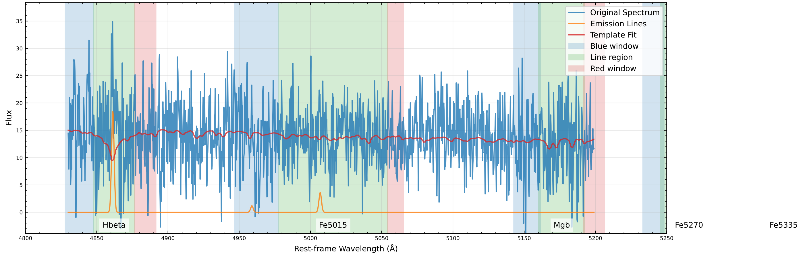
Original Data Comparison (v_star=-39.7 km/s, v_gas=-23.8 km/s)
