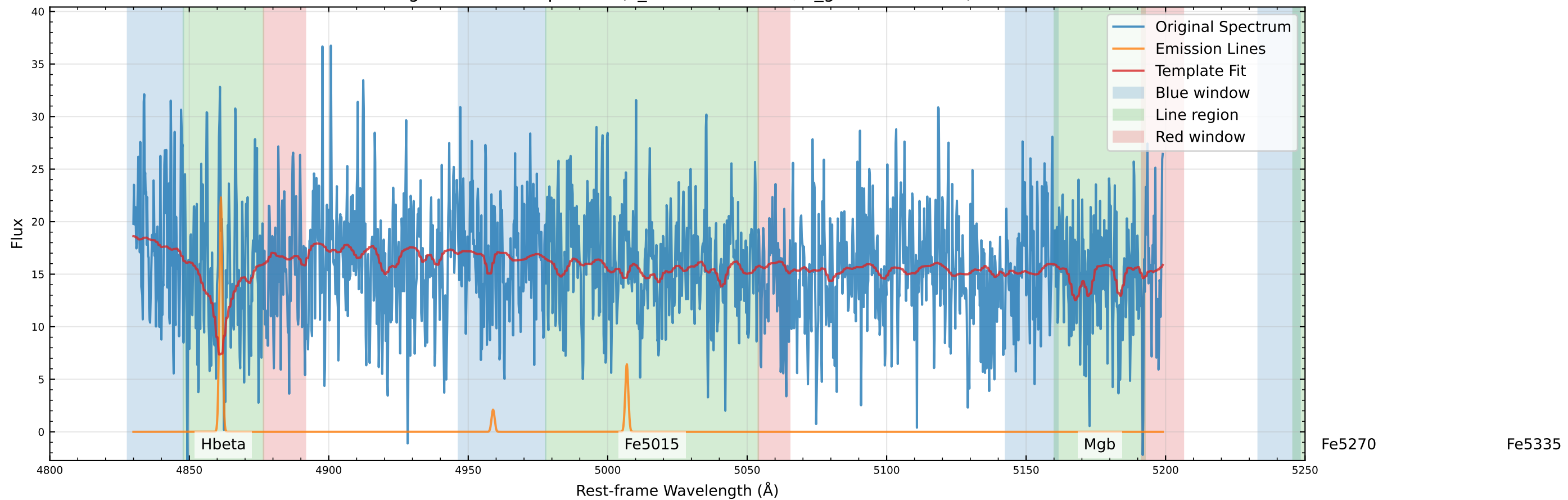
Original Data Comparison (v_star=-19.7 km/s, v_gas=-23.5 km/s)
