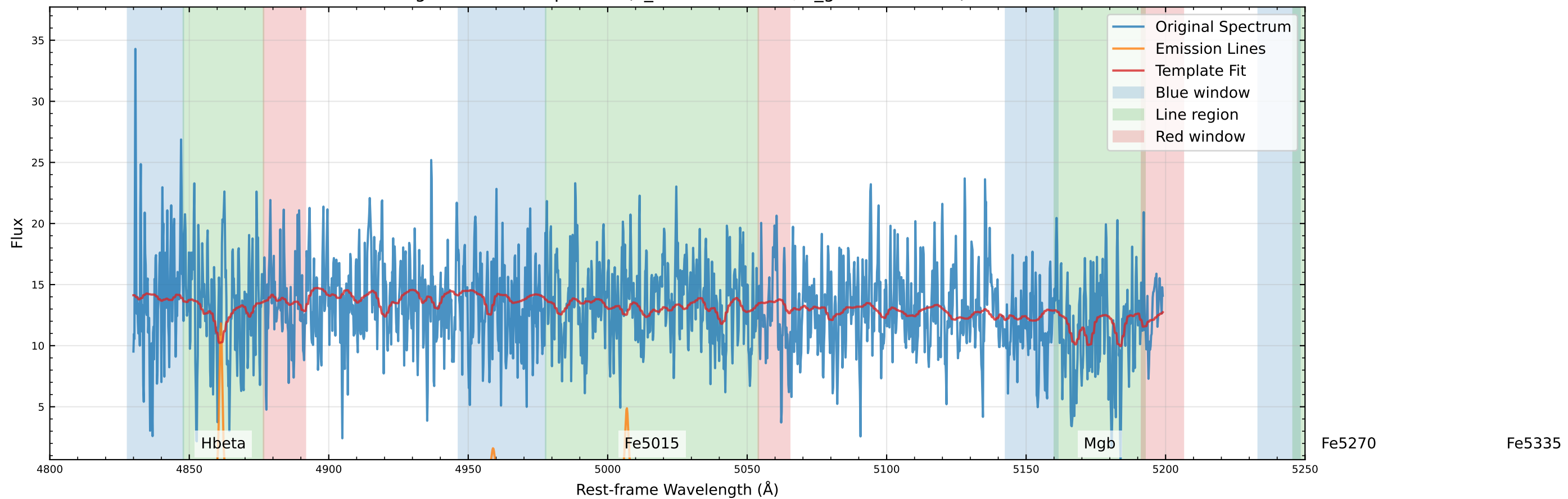
Original Data Comparison (v_star=28.2 km/s, v_gas=60.6 km/s)
