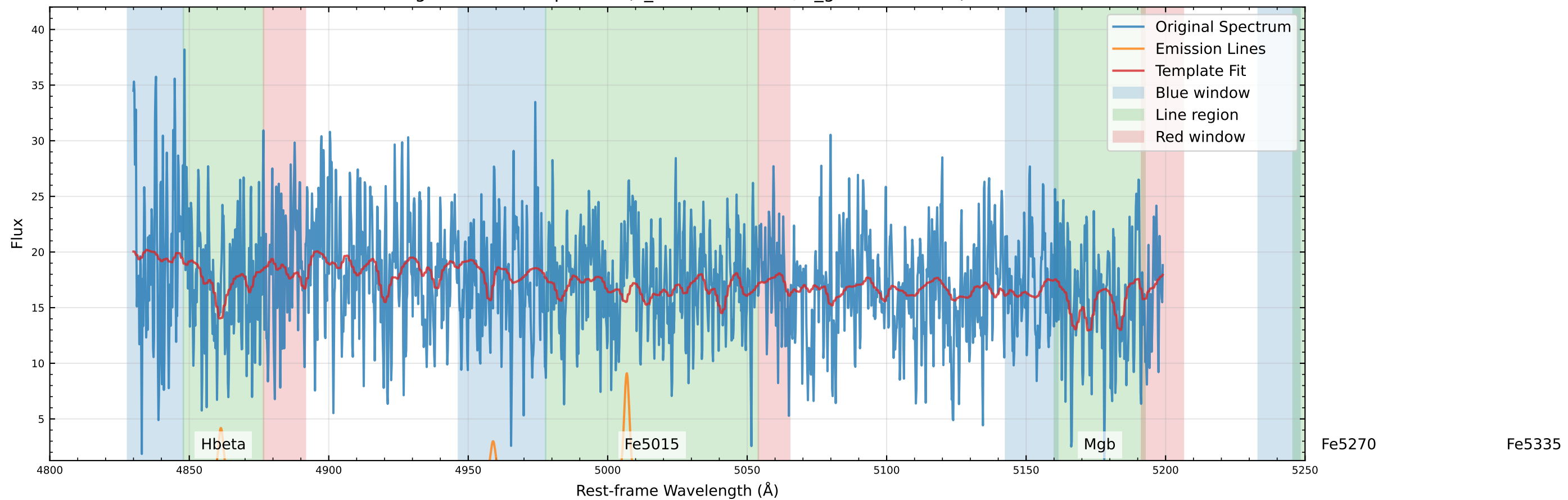
Original Data Comparison (v_star=11.4 km/s, v_gas=42.8 km/s)
