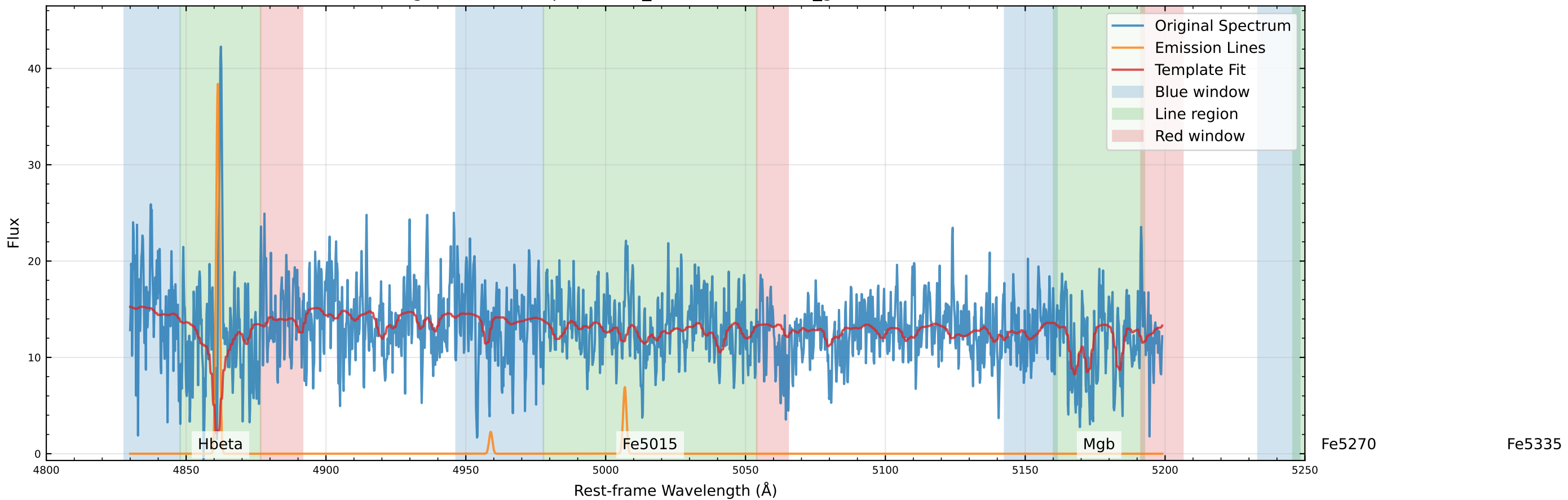
Original Data Comparison (v_star=51.1 km/s, v_gas=61.7 km/s)
