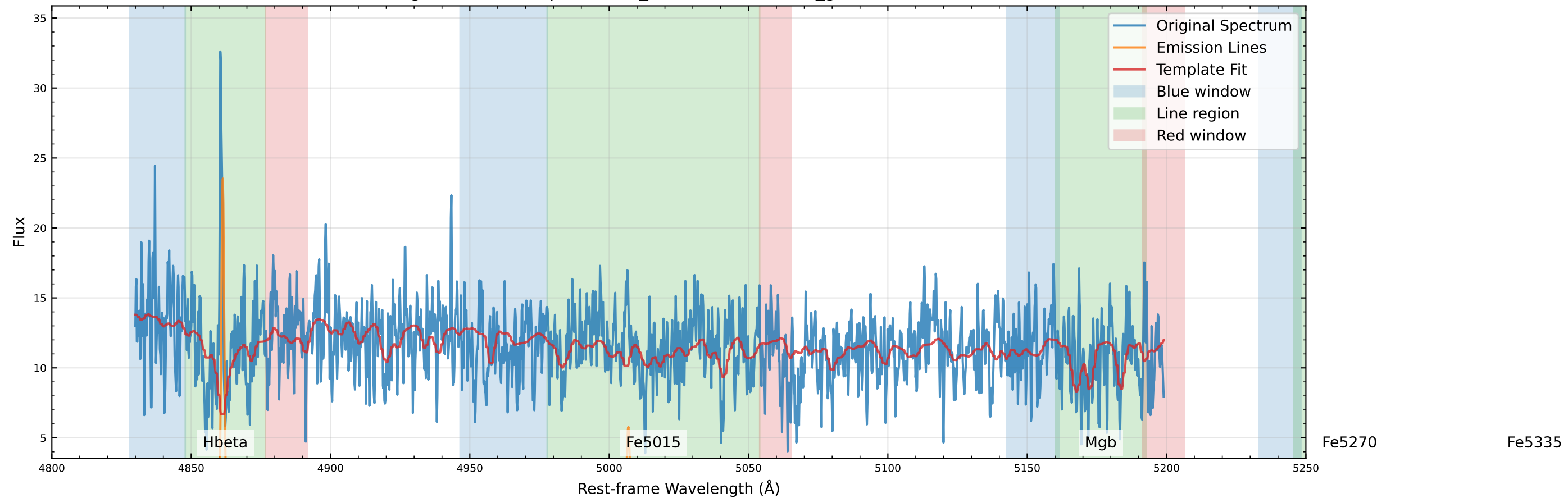
Original Data Comparison (v_star=-37.8 km/s, v_gas=-38.2 km/s)
