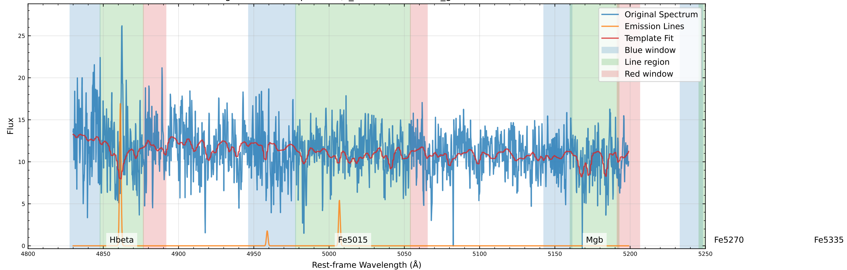
Original Data Comparison (v_star=30.3 km/s, v_gas=61.6 km/s)
