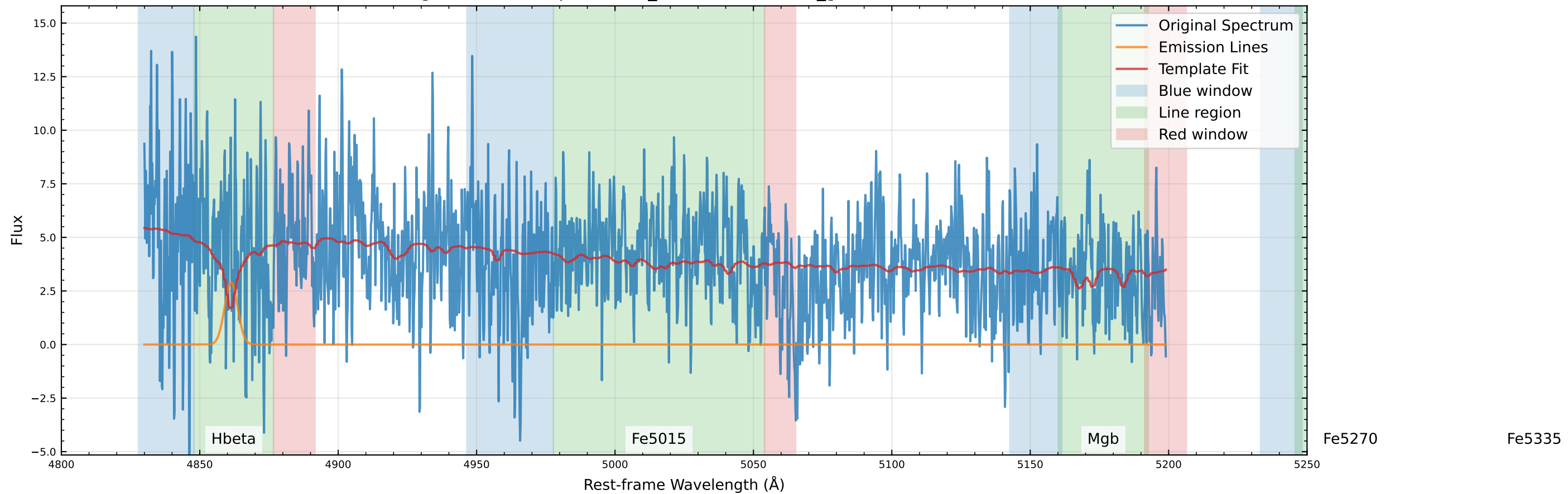
Original Data Comparison (v_star=50.2 km/s, v_gas=-30.6 km/s)
