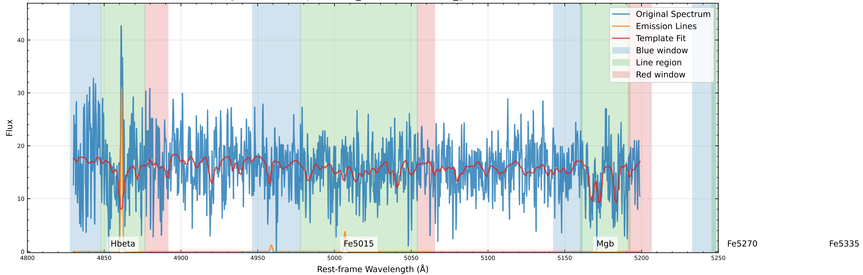
Original Data Comparison (v_star=-36.6 km/s, v_gas=1.3 km/s)
