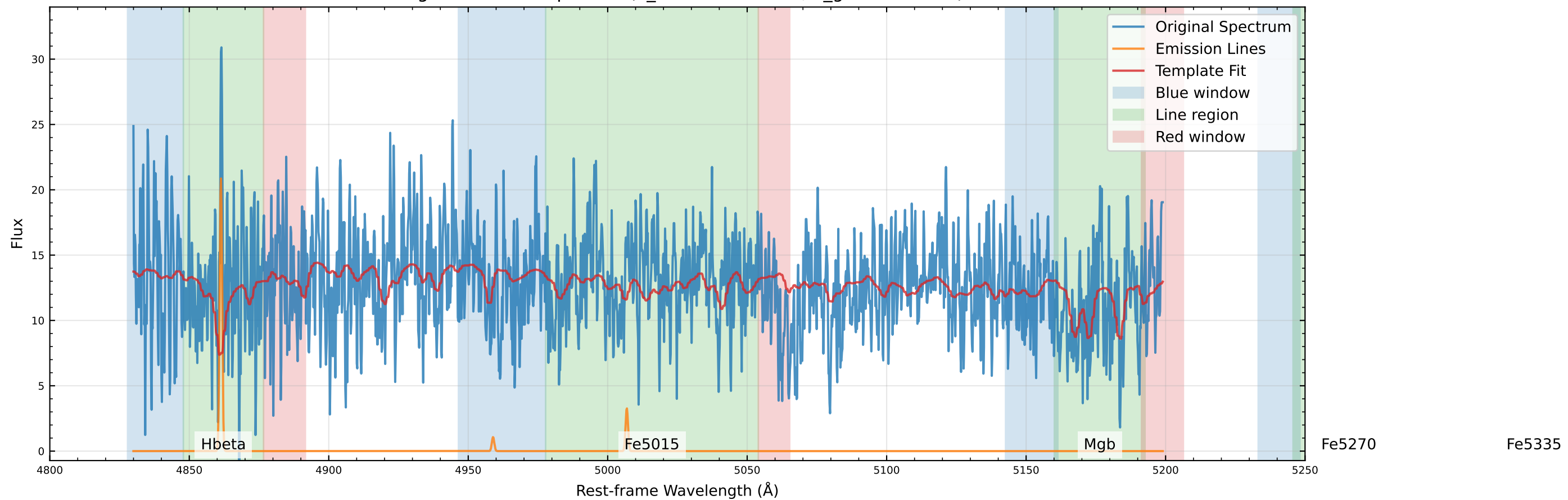
Original Data Comparison (v_star=-59.1 km/s, v_gas=7.2 km/s)
