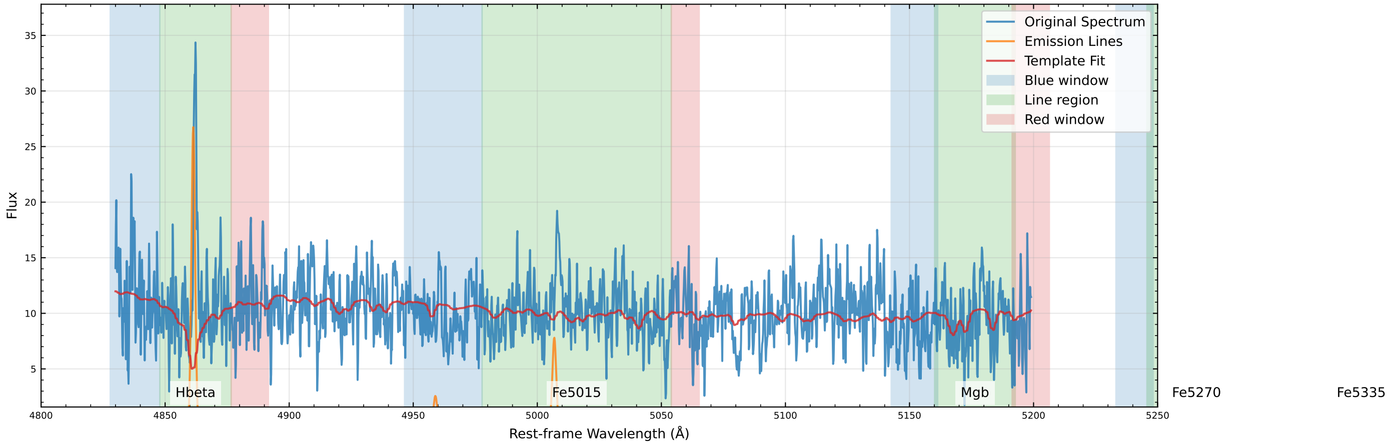
Original Data Comparison (v_star=70.9 km/s, v_gas=54.0 km/s)
