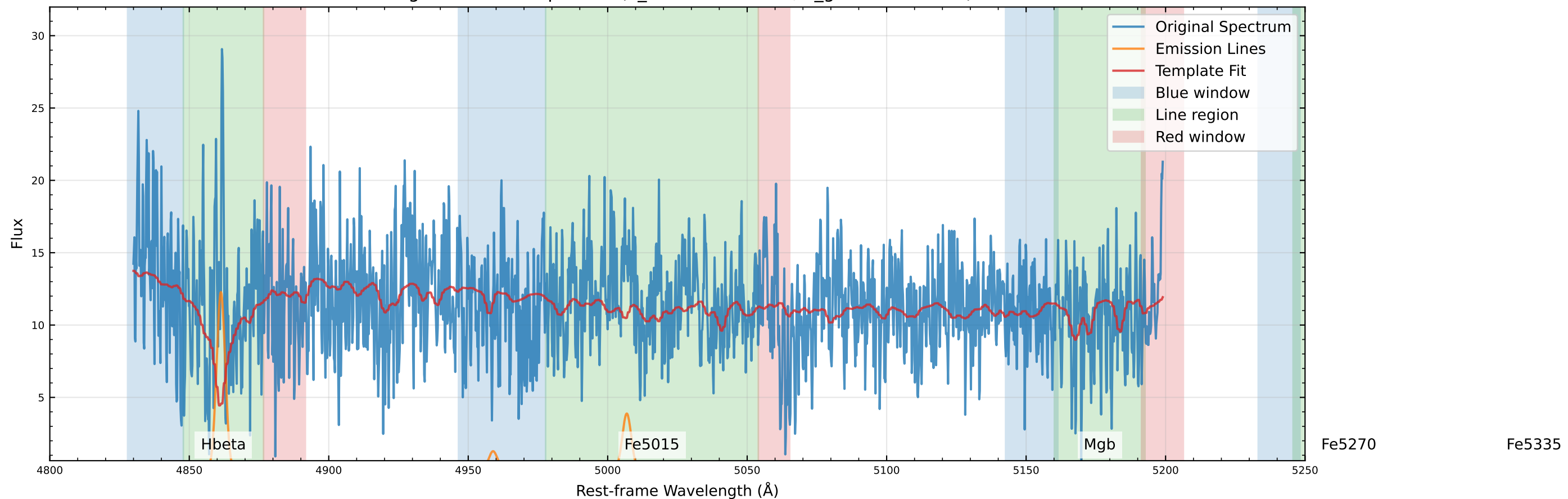
Original Data Comparison (v_star=-35.6 km/s, v_gas=-12.1 km/s)
