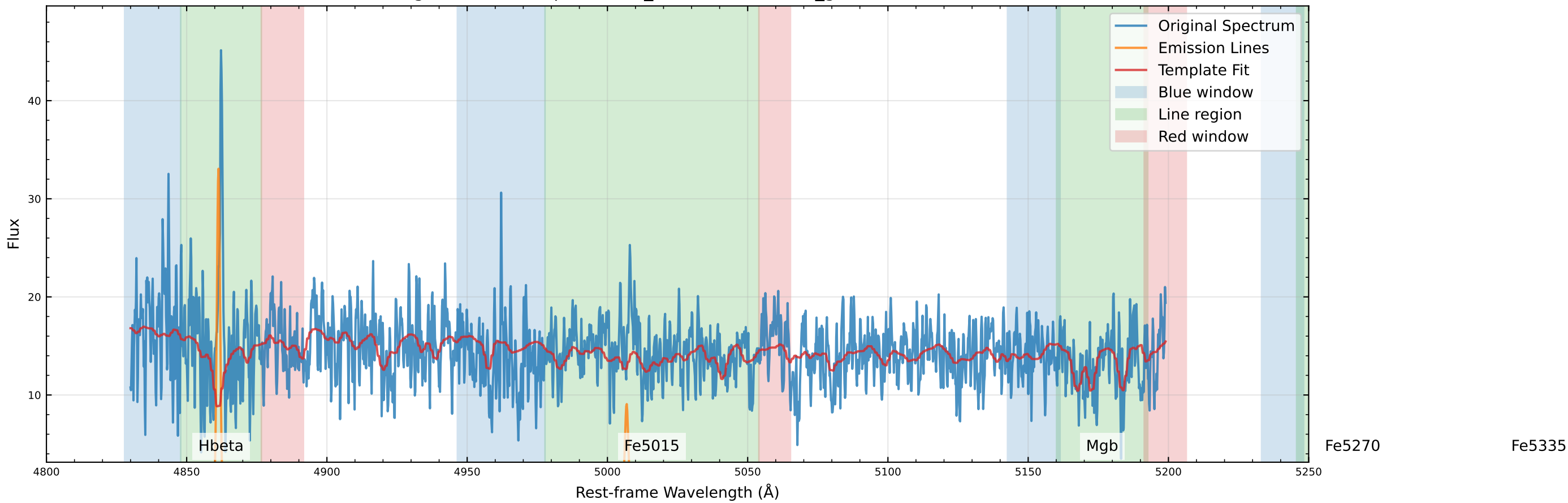
Original Data Comparison (v_star=37.1 km/s, v_gas=58.8 km/s)
