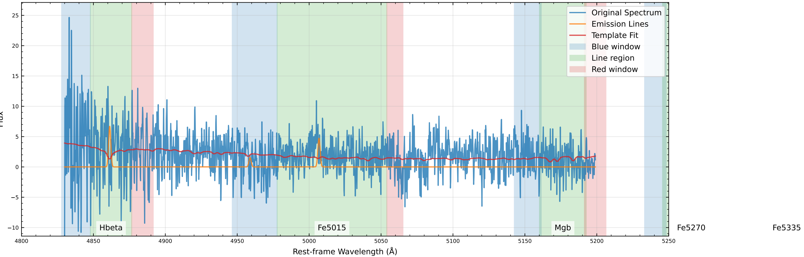
Original Data Comparison ( v_{\text{star}}=-80.6 km/s, v_{\text{gas}}=-114.8 km/s)
