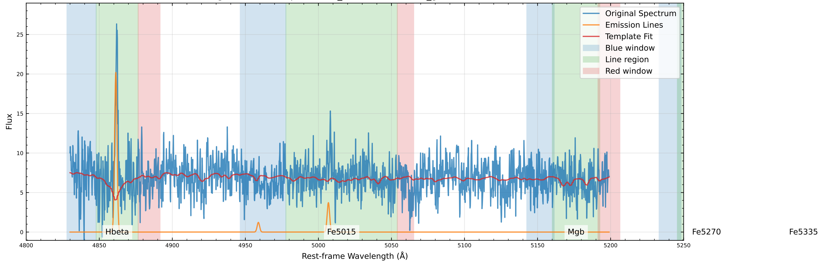
Original Data Comparison (v_star=41.9 km/s, v_gas=38.4 km/s)
