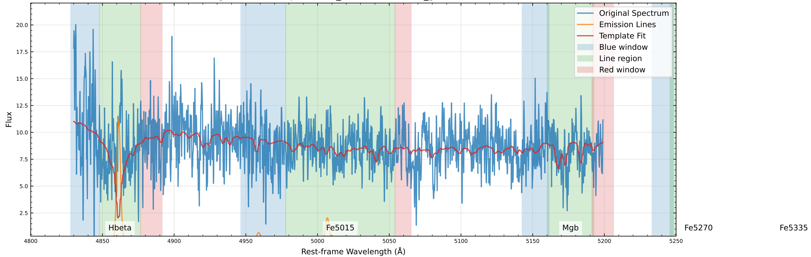
Original Data Comparison (v_star=86.9 km/s, v_gas=78.6 km/s)
