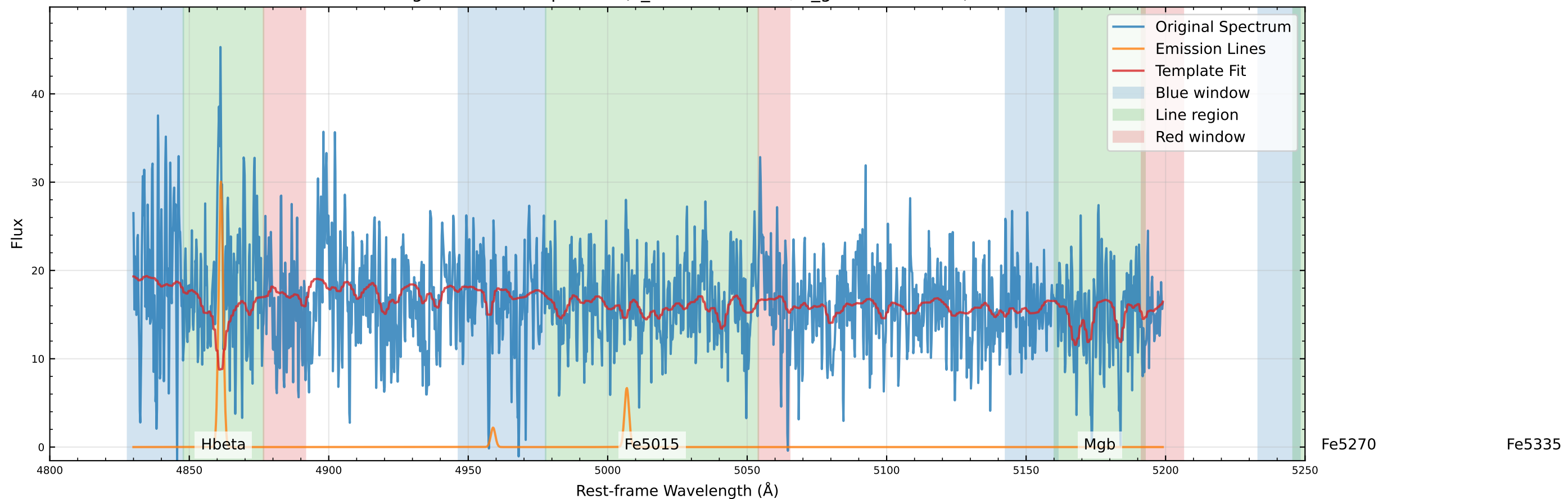
Original Data Comparison (v_star=15.8 km/s, v_gas=-22.0 km/s)
