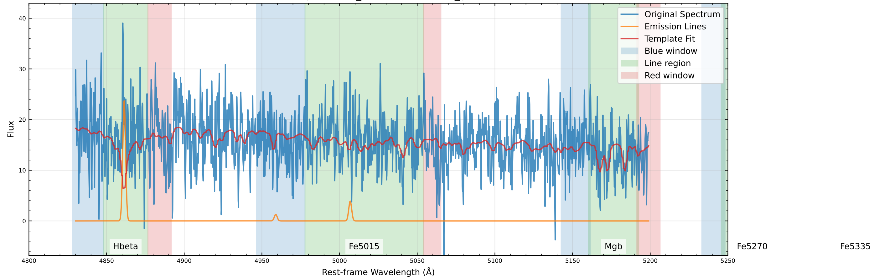
Original Data Comparison (v_star=-35.2 km/s, v_gas=-36.4 km/s)
