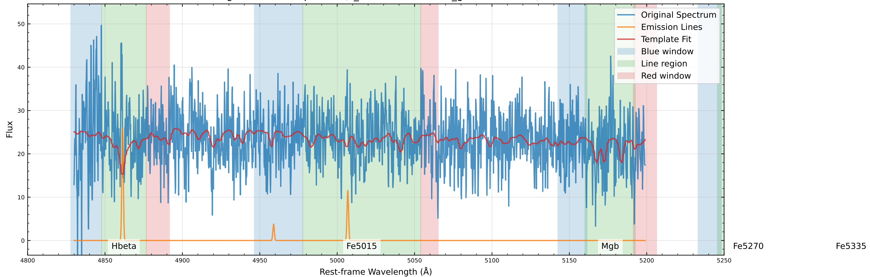
Original Data Comparison (v_star=-41.9 km/s, v_gas=-40.4 km/s)
