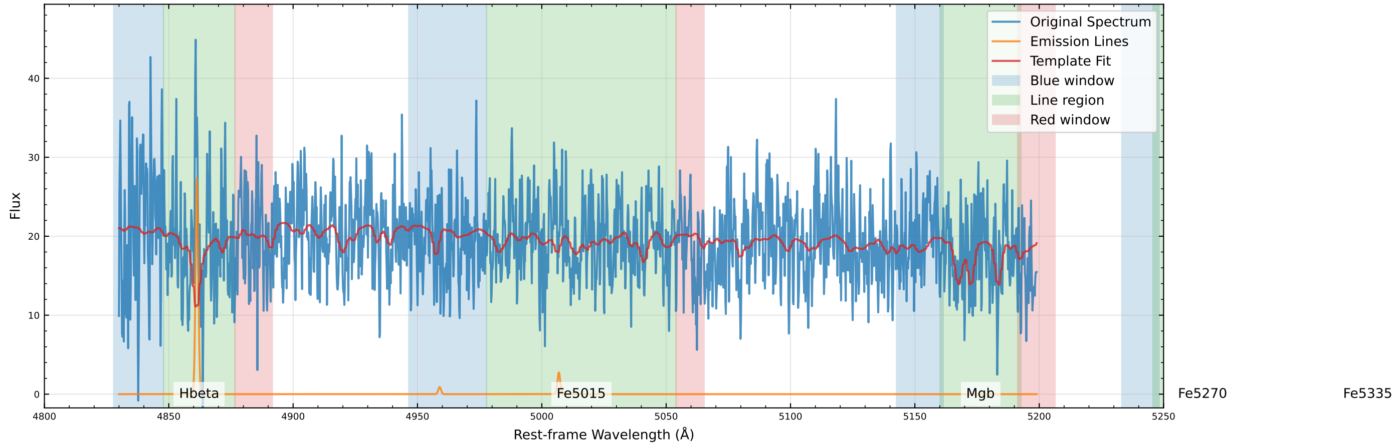
Original Data Comparison (v_star=-41.1 km/s, v_gas=-25.0 km/s)
