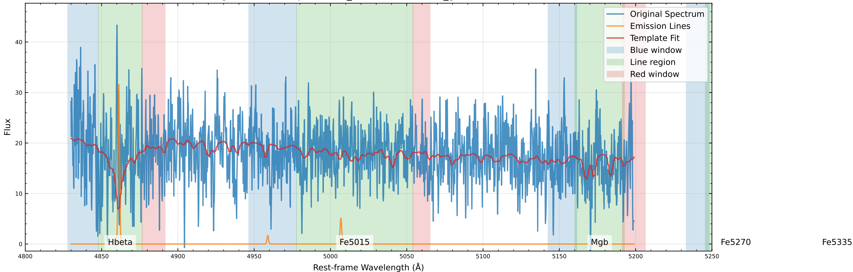
Original Data Comparison (v_star=-68.8 km/s, v_gas=-73.2 km/s)
