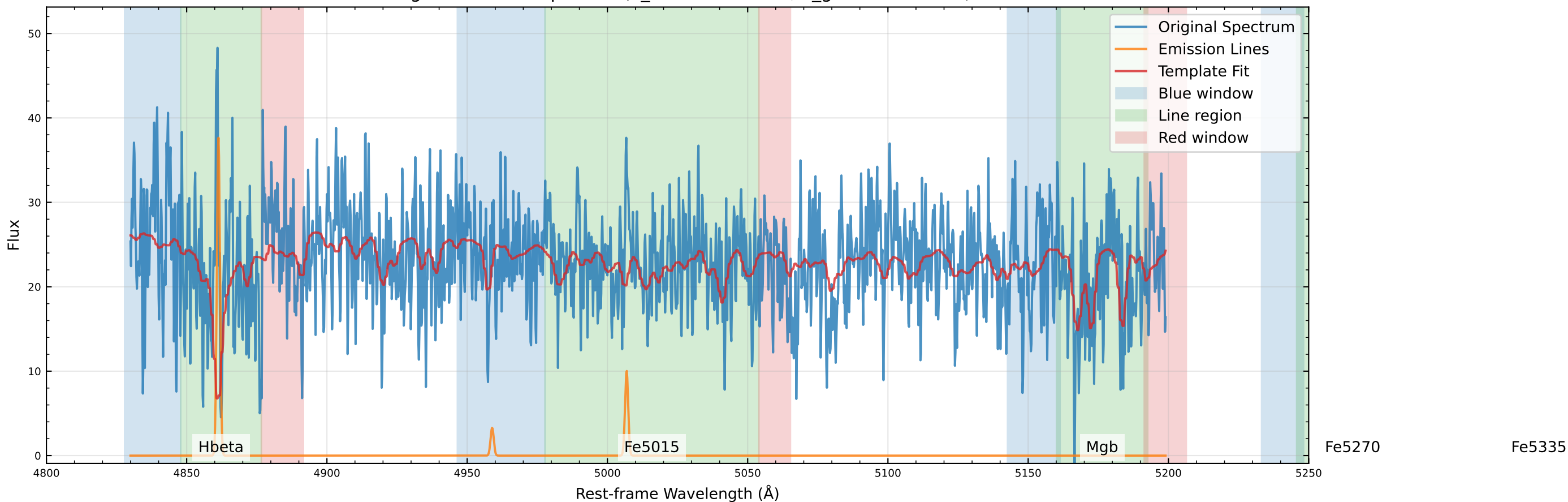
Original Data Comparison (v_star=10.8 km/s, v_gas=-28.2 km/s)
