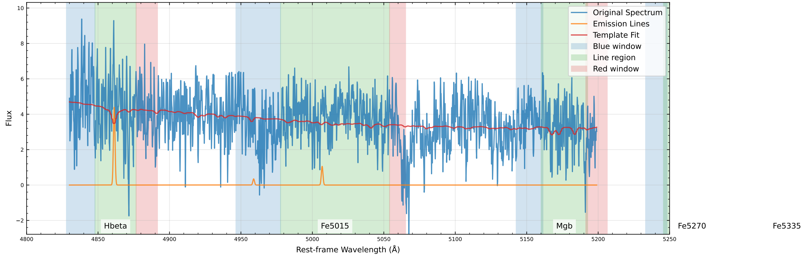
Original Data Comparison (v_star=-49.1 km/s, v_gas=-23.0 km/s)
