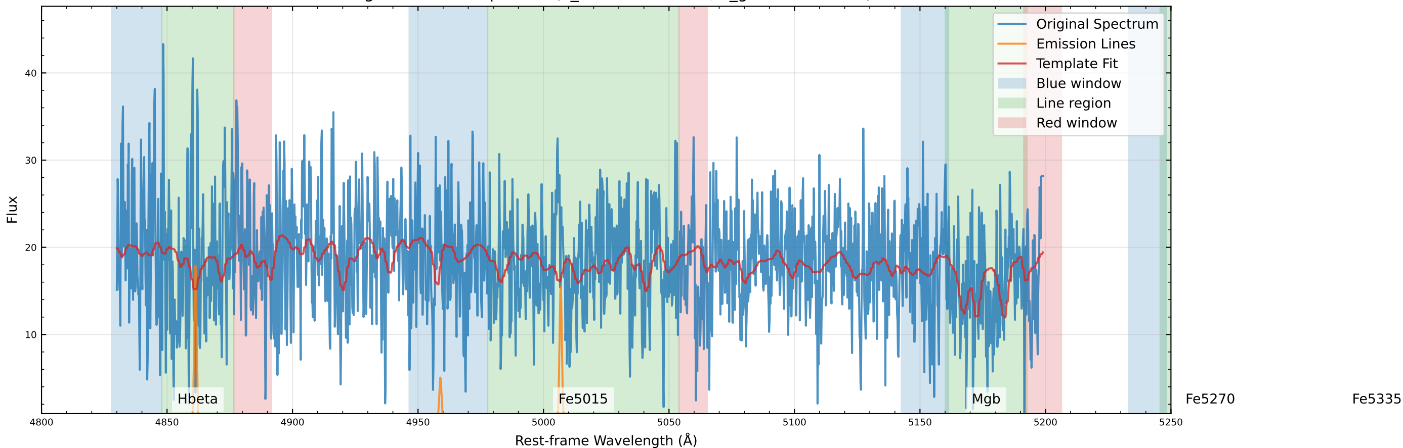
Original Data Comparison (v_star=-86.0 km/s, v_gas=-83.3 km/s)
