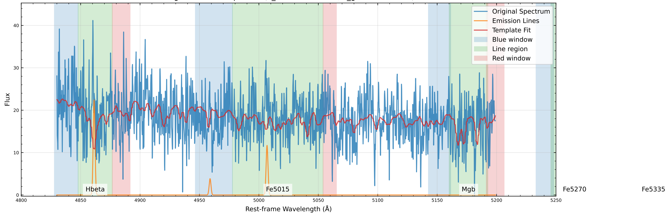
Original Data Comparison (v_star=-77.1 km/s, v_gas=-61.7 km/s)
