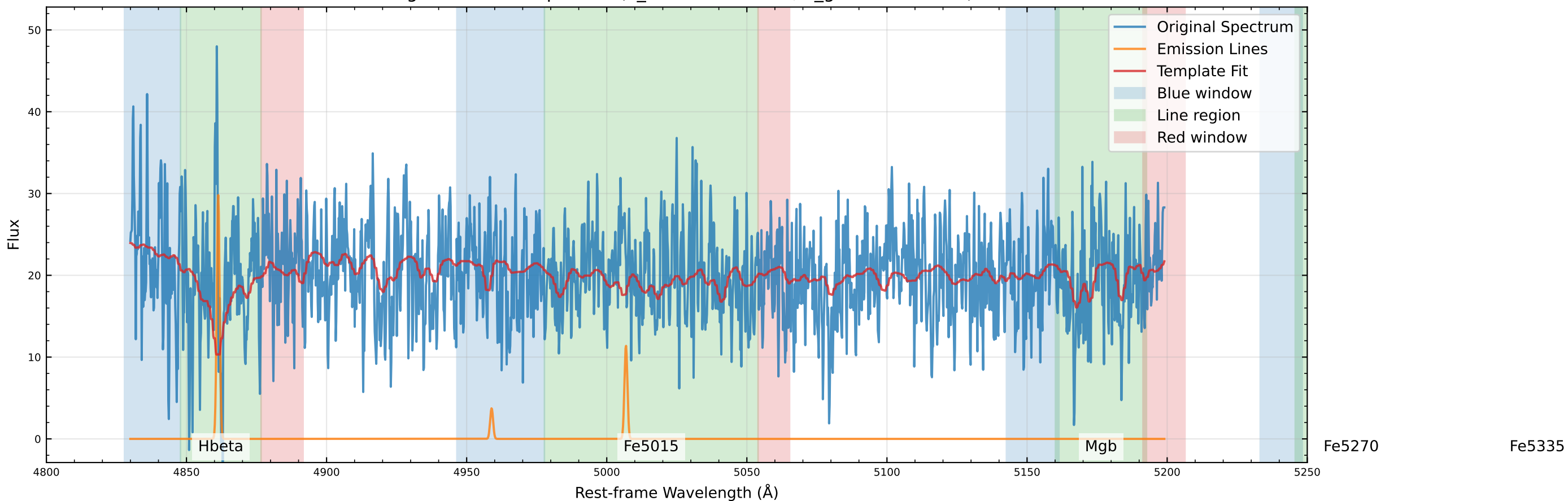
Original Data Comparison (v_star=-51.9 km/s, v_gas=-46.5 km/s)
