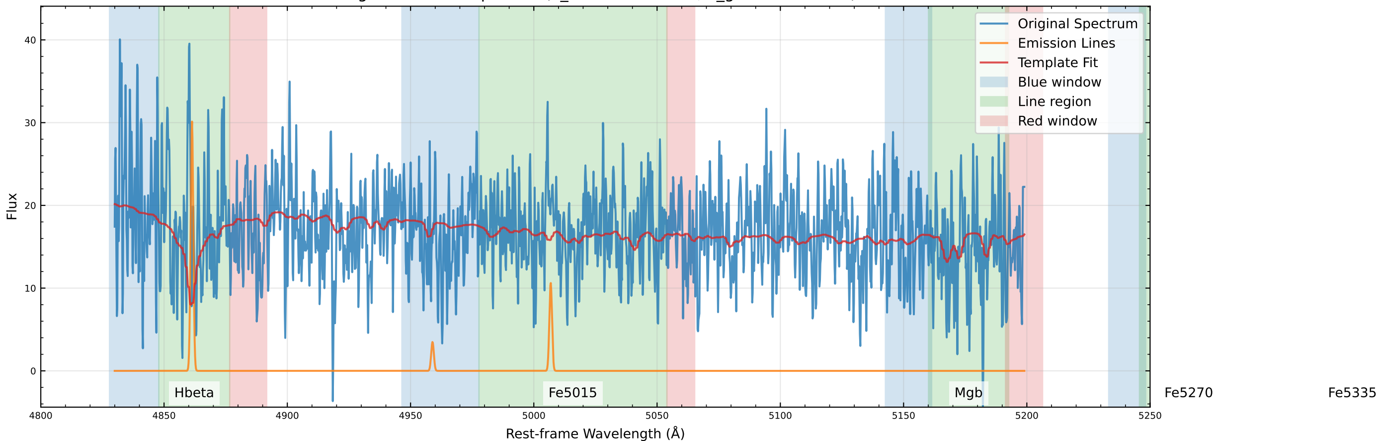
Original Data Comparison (v_star=-75.1 km/s, v_gas=-78.0 km/s)
