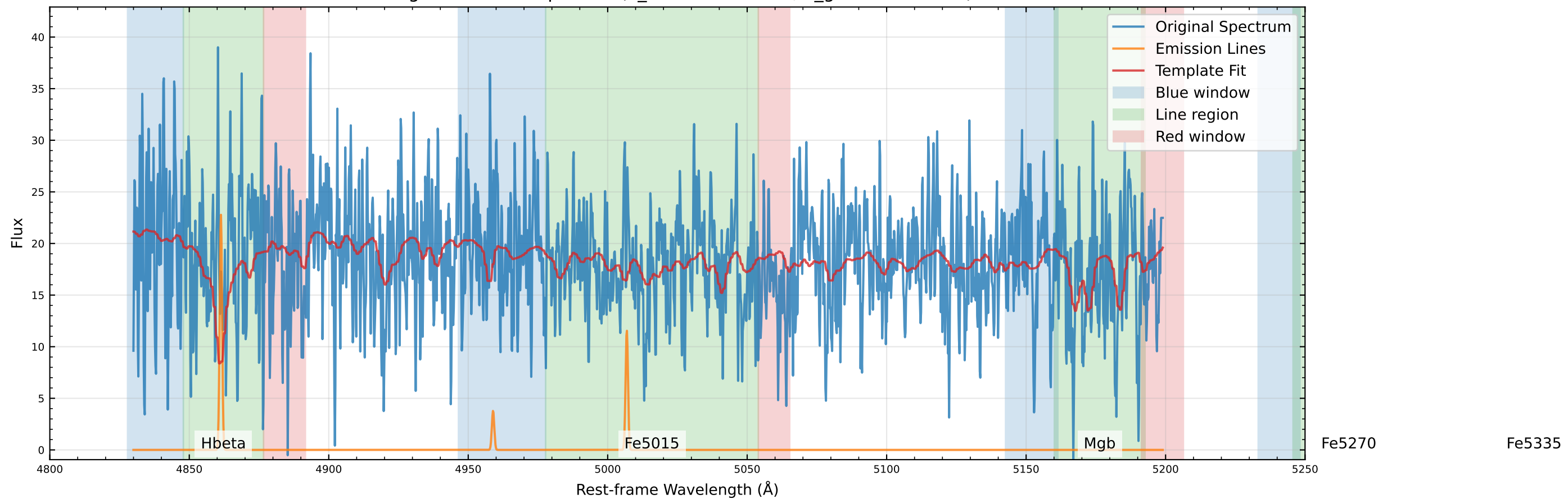
Original Data Comparison ( v_{\text{star}}=-80.6 km/s, v_{\text{gas}}=-65.2 km/s)
