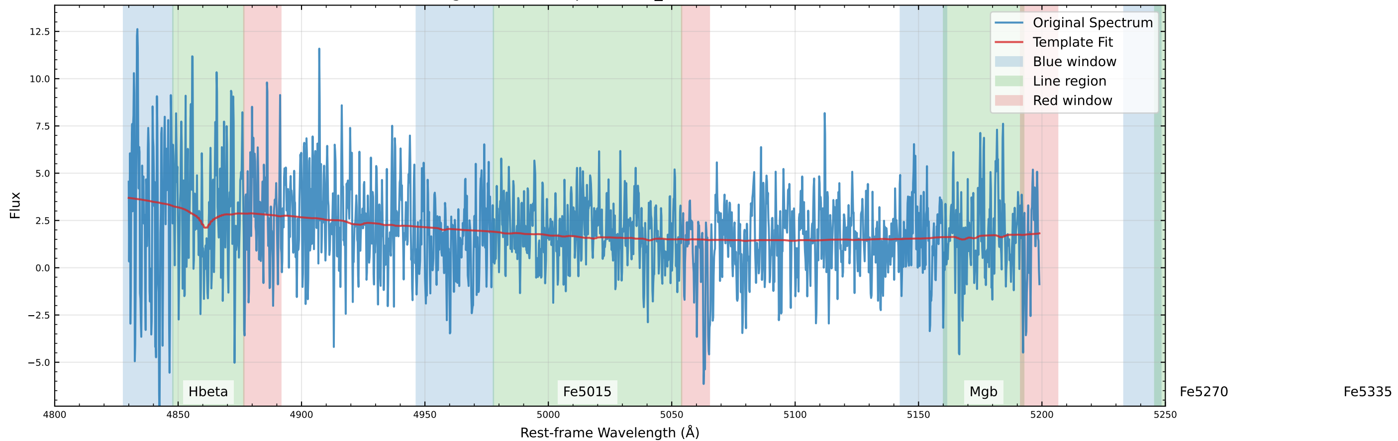
Original Data Comparison ( v_{\text{star}}=31.3 km/s)
