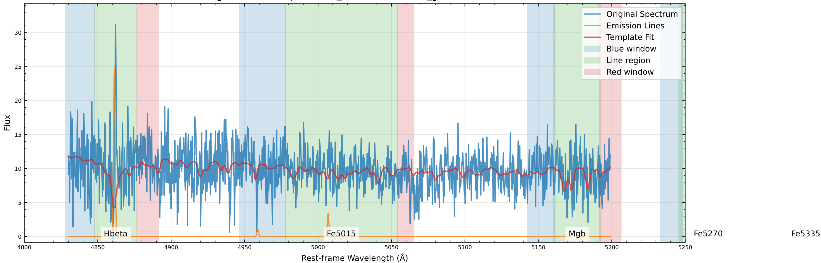
Original Data Comparison (v_star=56.7 km/s, v_gas=46.5 km/s)
