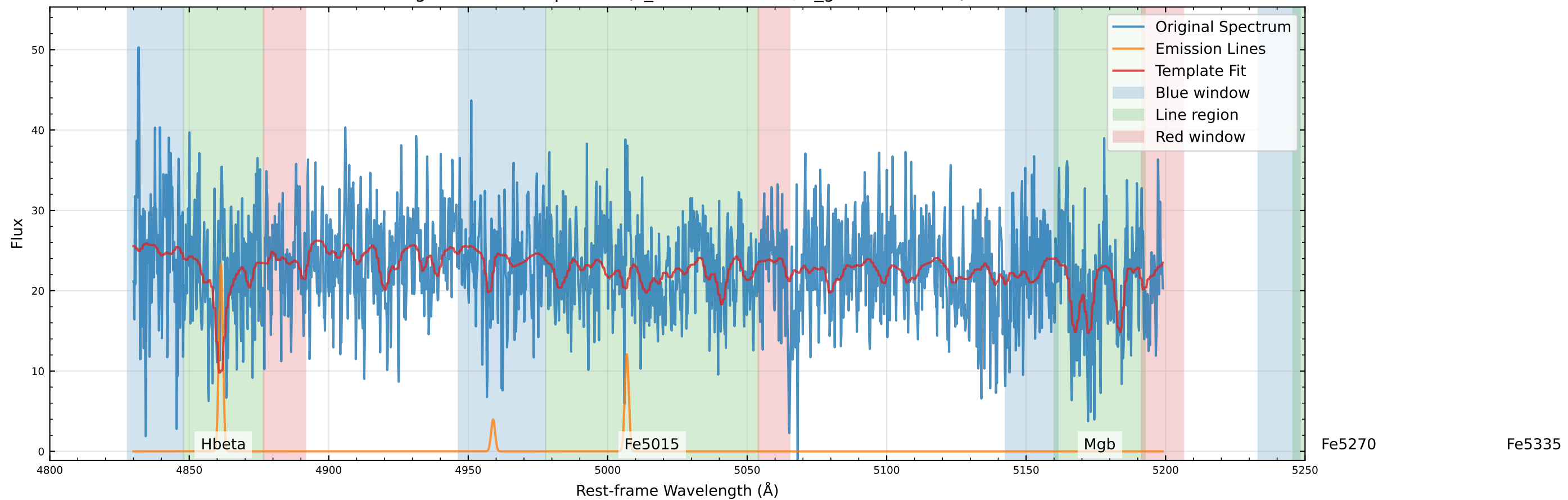
Original Data Comparison (v_star=21.9 km/s, v_gas=20.1 km/s)
